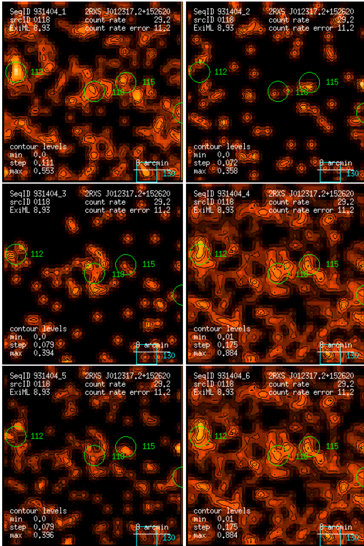
Figure 118: RASS 931404: detection 0118: band rate images, Gaussian filter: (1) PSPC channels 11 – 41, (2) 52 – 90, (3) 91 – 201, (4) 11 – 235, (5) 52 – 201, (6) 11 – 201. Broad band rates in counts/ks. Band rate contour levels in counts/ks/arcmin 2 .
