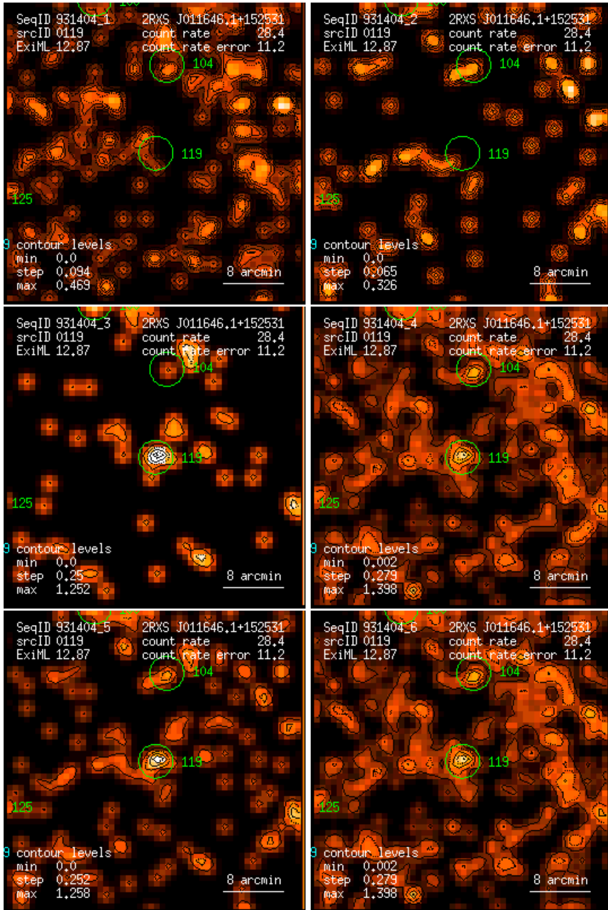
Figure 119: RASS 931404: detection 0119: band rate images, Gaussian filter: (1) PSPC channels 11 – 41, (2) 52 – 90, (3) 91 – 201, (4) 11 – 235, (5) 52 – 201, (6) 11 – 201. Broad band rates in counts/ks. Band rate contour levels in counts/ks/arcmin 2 .
