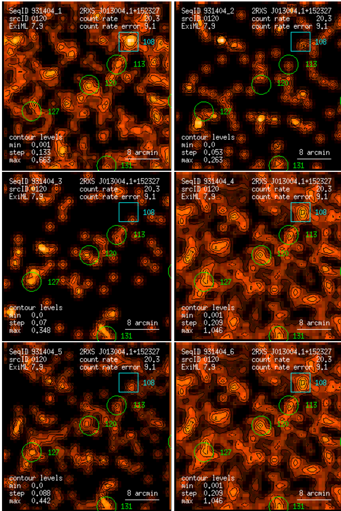
Figure 120: RASS 931404: detection 0120: band rate images, Gaussian filter: (1) PSPC channels 11 – 41, (2) 52 – 90, (3) 91 – 201, (4) 11 – 235, (5) 52 – 201, (6) 11 – 201. Broad band rates in counts/ks. Band rate contour levels in counts/ks/arcmin 2 .
