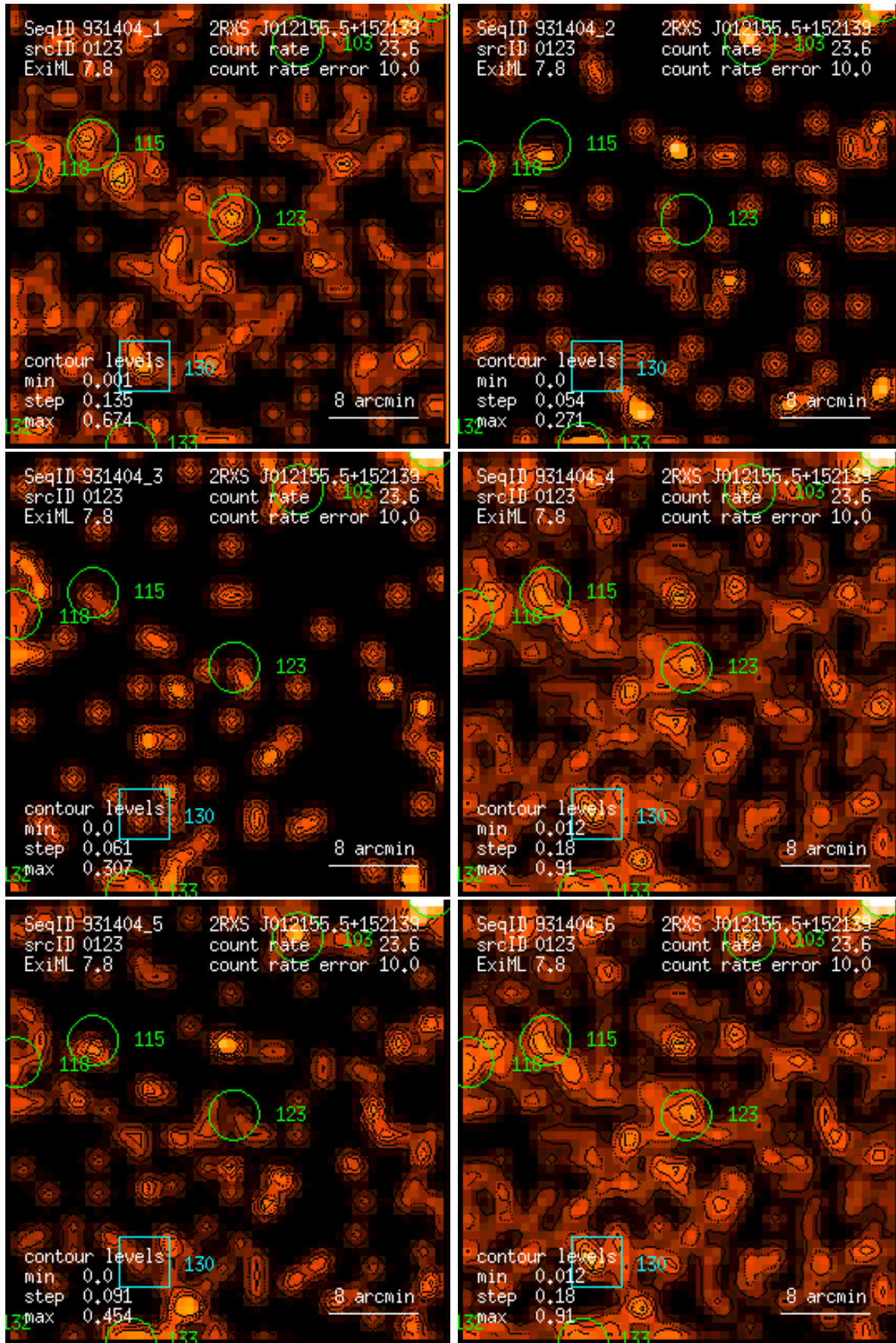
Figure 123: RASS 931404: detection 0123: band rate images, Gaussian filter: (1) PSPC channels 11 – 41, (2) 52 – 90, (3) 91 – 201, (4) 11 – 235, (5) 52 – 201, (6) 11 – 201. Broad band rates in counts/ks. Band rate contour levels in counts/ks/arcmin 2 .
