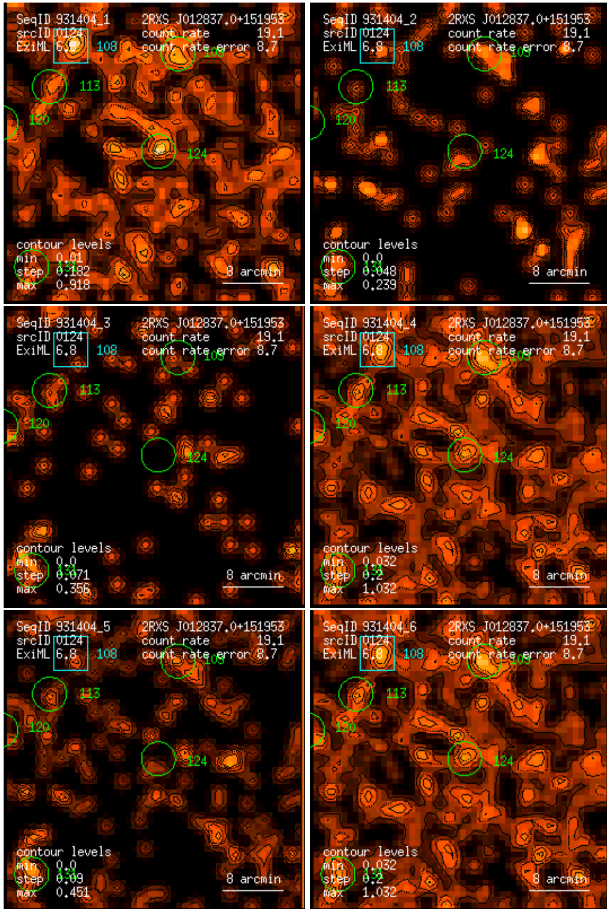
Figure 124: RASS 931404: detection 0124: band rate images, Gaussian filter: (1) PSPC channels 11 – 41, (2) 52 – 90, (3) 91 – 201, (4) 11 – 235, (5) 52 – 201, (6) 11 – 201. Broad band rates in counts/ks. Band rate contour levels in counts/ks/arcmin 2 .
