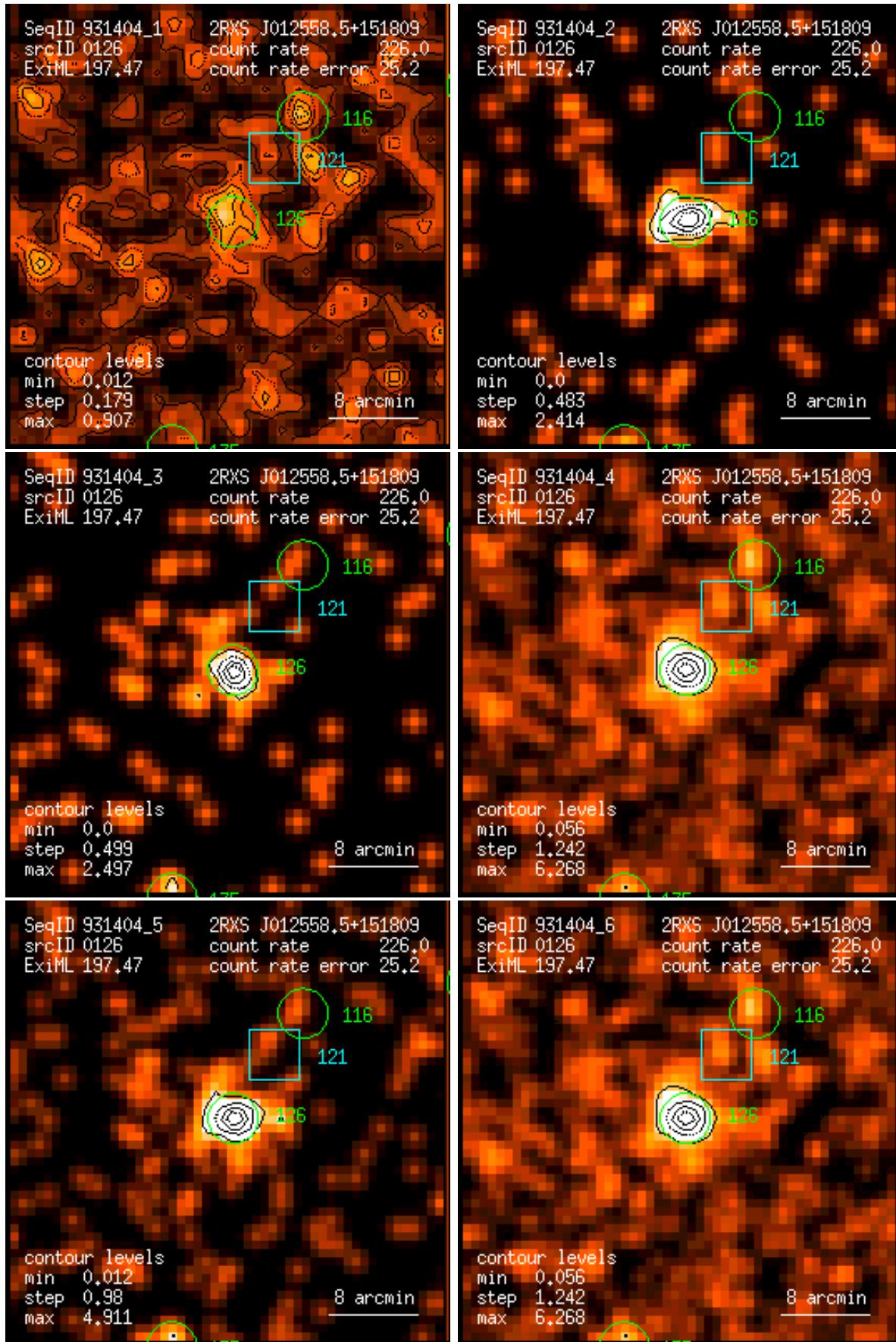
Figure 126: RASS 931404: detection 0126: band rate images, Gaussian filter: (1) PSPC channels 11 – 41, (2) 52 – 90, (3) 91 – 201, (4) 11 – 235, (5) 52 – 201, (6) 11 – 201. Broad band rates in counts/ks. Band rate contour levels in counts/ks/arcmin 2 .
