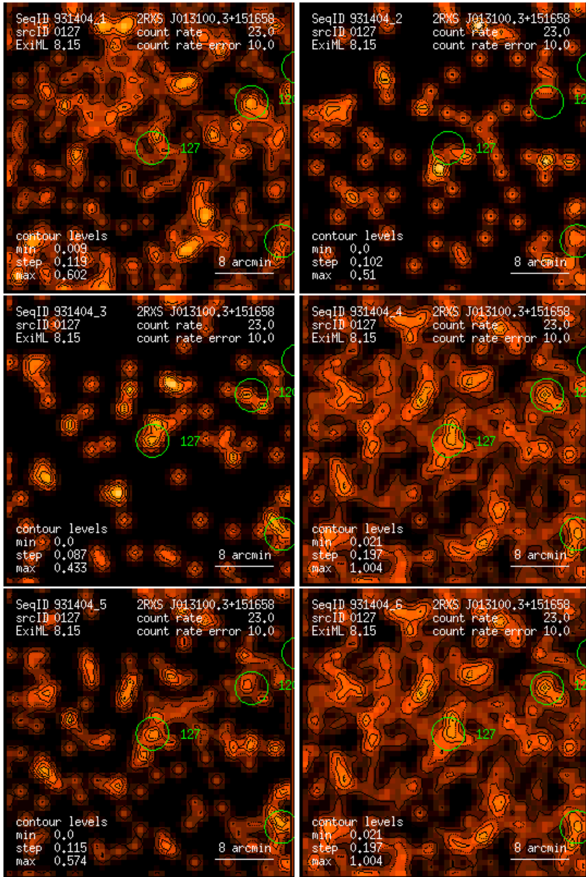
Figure 127: RASS 931404: detection 0127: band rate images, Gaussian filter: (1) PSPC channels 11 – 41, (2) 52 – 90, (3) 91 – 201, (4) 11 – 235, (5) 52 – 201, (6) 11 – 201. Broad band rates in counts/ks. Band rate contour levels in counts/ks/arcmin 2 .
