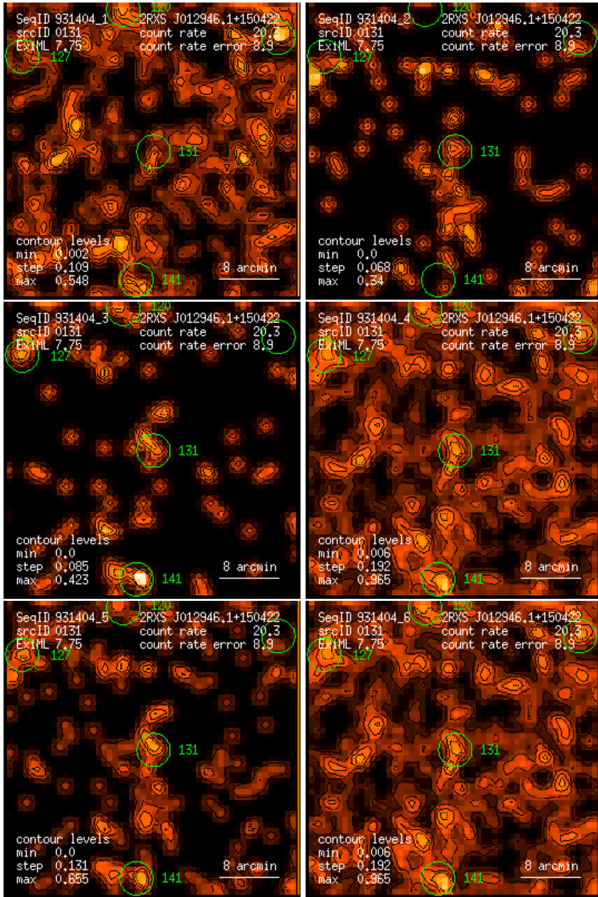
Figure 131: RASS 931404: detection 0131: band rate images, Gaussian filter: (1) PSPC channels 11 – 41, (2) 52 – 90, (3) 91 – 201, (4) 11 – 235, (5) 52 – 201, (6) 11 – 201. Broad band rates in counts/ks. Band rate contour levels in counts/ks/arcmin 2 .
