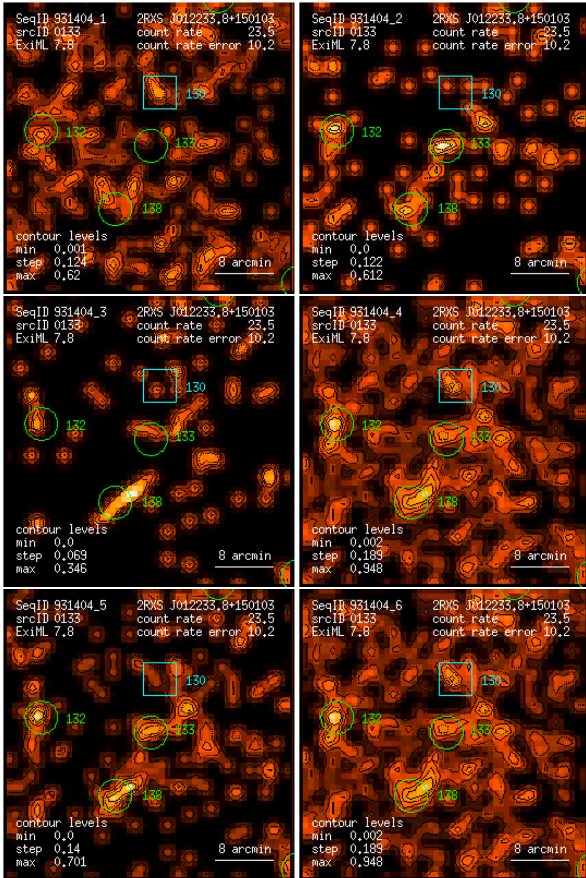
Figure 133: RASS 931404: detection 0133: band rate images, Gaussian filter: (1) PSPC channels 11 – 41, (2) 52 – 90, (3) 91 – 201, (4) 11 – 235, (5) 52 – 201, (6) 11 – 201. Broad band rates in counts/ks. Band rate contour levels in counts/ks/arcmin 2 .
