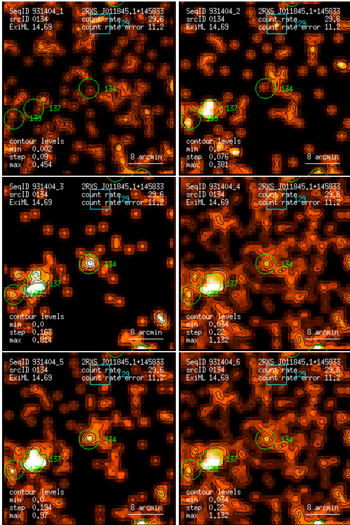
Figure 134: RASS 931404: detection 0134: band rate images, Gaussian filter: (1) PSPC channels 11 – 41, (2) 52 – 90, (3) 91 – 201, (4) 11 – 235, (5) 52 – 201, (6) 11 – 201. Broad band rates in counts/ks. Band rate contour levels in counts/ks/arcmin 2 .
