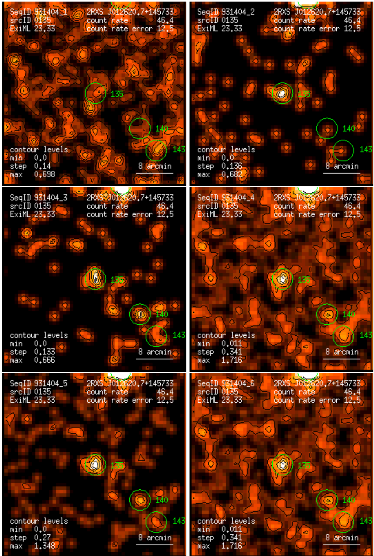
Figure 135: RASS 931404: detection 0135: band rate images, Gaussian filter: (1) PSPC channels 11 – 41, (2) 52 – 90, (3) 91 – 201, (4) 11 – 235, (5) 52 – 201, (6) 11 – 201. Broad band rates in counts/ks. Band rate contour levels in counts/ks/arcmin 2 .
