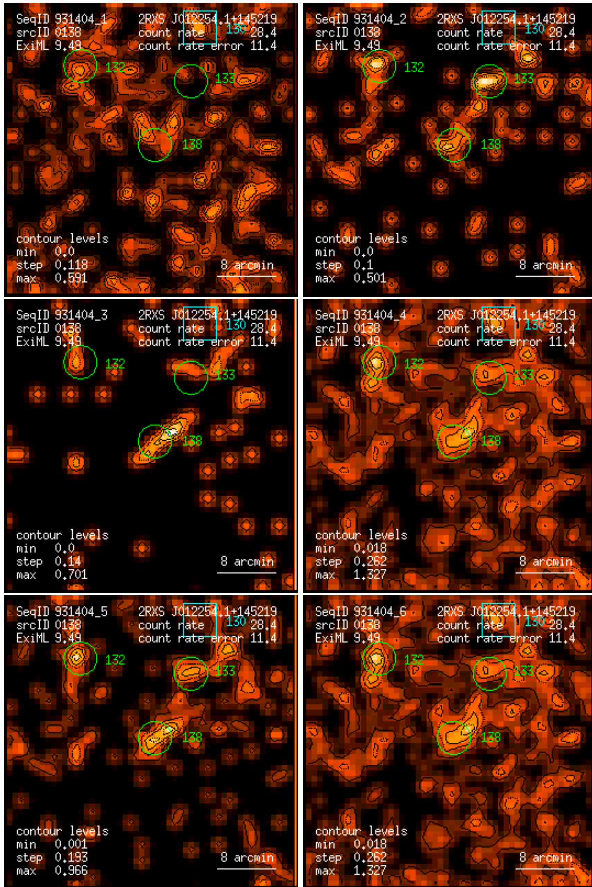
Figure 138: RASS 931404: detection 0138: band rate images, Gaussian filter: (1) PSPC channels 11 – 41, (2) 52 – 90, (3) 91 – 201, (4) 11 – 235, (5) 52 – 201, (6) 11 – 201. Broad band rates in counts/ks. Band rate contour levels in counts/ks/arcmin 2 .
