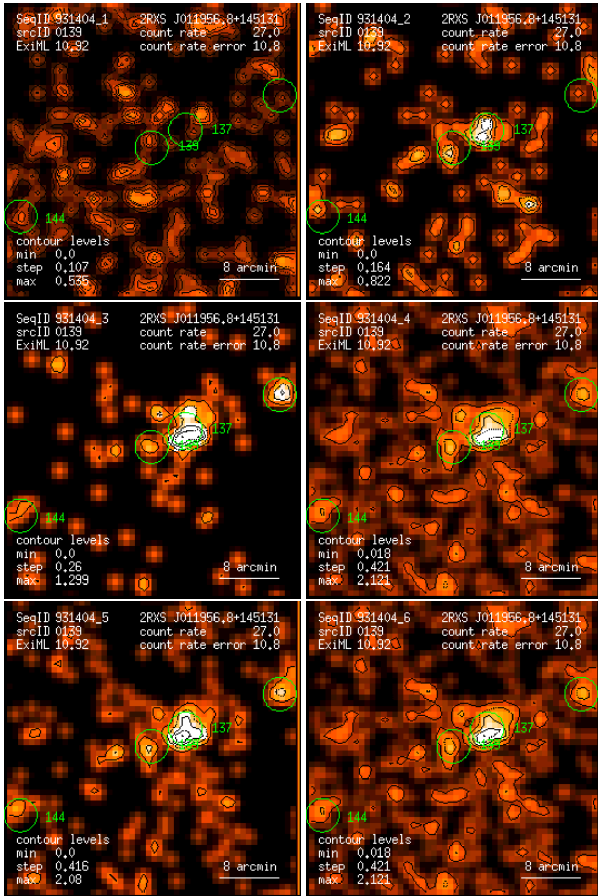
Figure 139: RASS 931404: detection 0139: band rate images, Gaussian filter: (1) PSPC channels 11 – 41, (2) 52 – 90, (3) 91 – 201, (4) 11 – 235, (5) 52 – 201, (6) 11 – 201. Broad band rates in counts/ks. Band rate contour levels in counts/ks/arcmin 2 .
