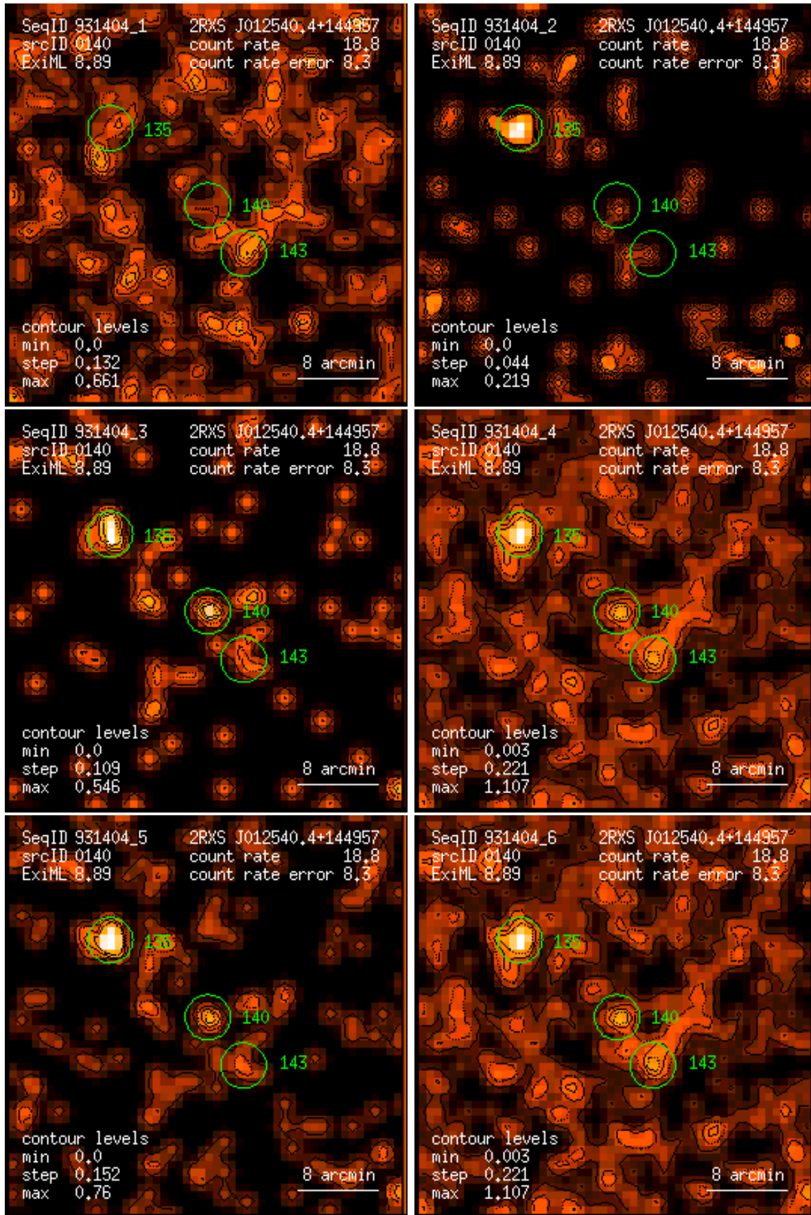
Figure 140: RASS 931404: detection 0140: band rate images, Gaussian filter: (1) PSPC channels 11 – 41, (2) 52 – 90, (3) 91 – 201, (4) 11 – 235, (5) 52 – 201, (6) 11 – 201. Broad band rates in counts/ks. Band rate contour levels in counts/ks/arcmin 2 .
