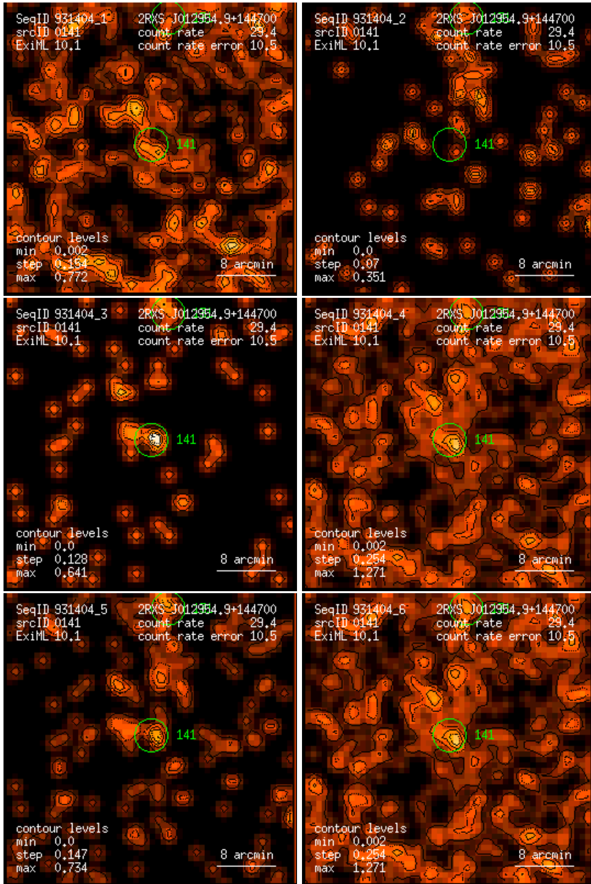
Figure 141: RASS 931404: detection 0141: band rate images, Gaussian filter: (1) PSPC channels 11 – 41, (2) 52 – 90, (3) 91 – 201, (4) 11 – 235, (5) 52 – 201, (6) 11 – 201. Broad band rates in counts/ks. Band rate contour levels in counts/ks/arcmin 2 .
