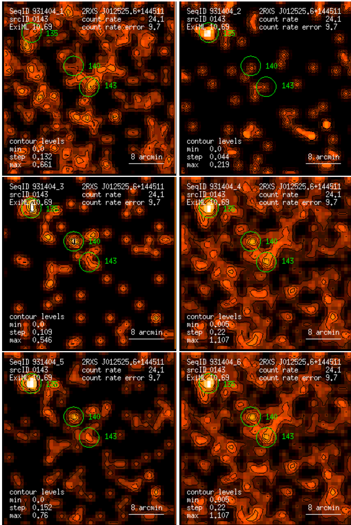
Figure 143: RASS 931404: detection 0143: band rate images, Gaussian filter: (1) PSPC channels 11 – 41, (2) 52 – 90, (3) 91 – 201, (4) 11 – 235, (5) 52 – 201, (6) 11 – 201. Broad band rates in counts/ks. Band rate contour levels in counts/ks/arcmin 2 .
