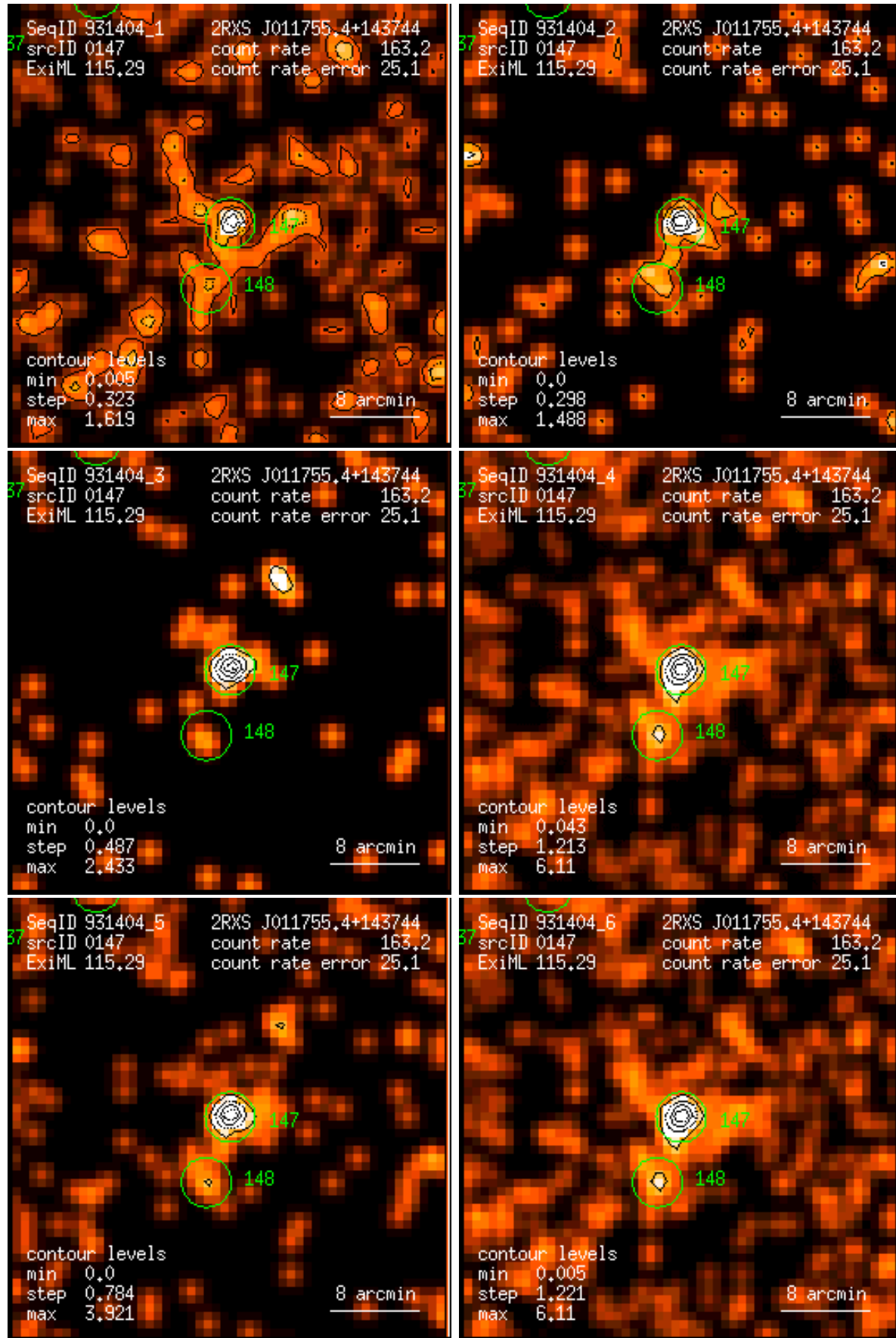
Figure 147: RASS 931404: detection 0147: band rate images, Gaussian filter: (1) PSPC channels 11 – 41, (2) 52 – 90, (3) 91 – 201, (4) 11 – 235, (5) 52 – 201, (6) 11 – 201. Broad band rates in counts/ks. Band rate contour levels in counts/ks/arcmin 2 .
