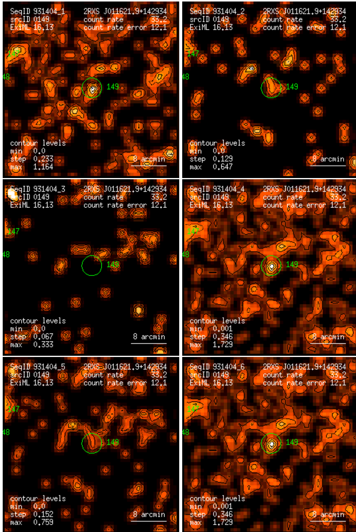
Figure 149: RASS 931404: detection 0149: band rate images, Gaussian filter: (1) PSPC channels 11 – 41, (2) 52 – 90, (3) 91 – 201, (4) 11 – 235, (5) 52 – 201, (6) 11 – 201. Broad band rates in counts/ks. Band rate contour levels in counts/ks/arcmin 2 .
