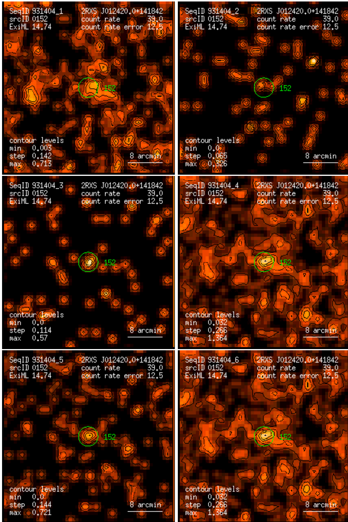
Figure 152: RASS 931404: detection 0152: band rate images, Gaussian filter: (1) PSPC channels 11 – 41, (2) 52 – 90, (3) 91 – 201, (4) 11 – 235, (5) 52 – 201, (6) 11 – 201. Broad band rates in counts/ks. Band rate contour levels in counts/ks/arcmin 2 .
