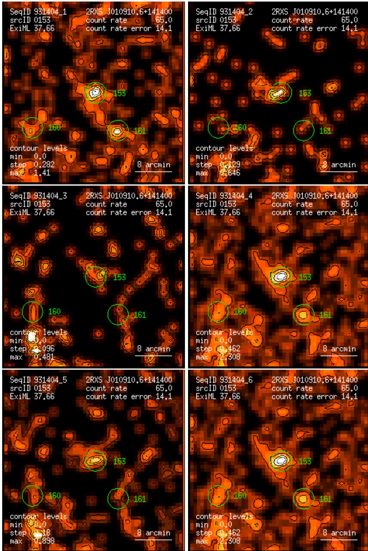
Figure 153: RASS 931404: detection 0153: band rate images, Gaussian filter: (1) PSPC channels 11 – 41, (2) 52 – 90, (3) 91 – 201, (4) 11 – 235, (5) 52 – 201, (6) 11 – 201. Broad band rates in counts/ks. Band rate contour levels in counts/ks/arcmin 2 .
