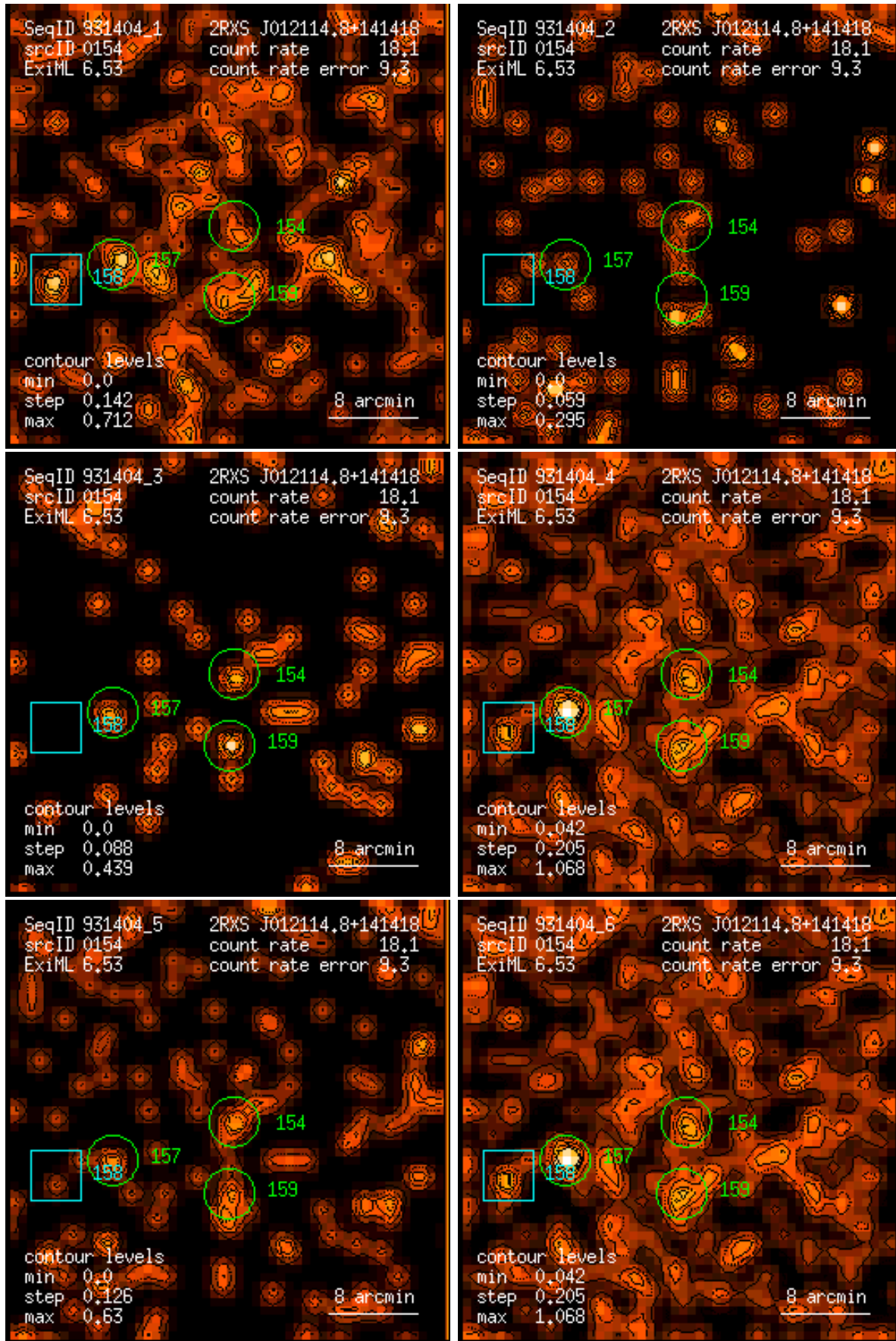
Figure 154: RASS 931404: detection 0154: band rate images, Gaussian filter: (1) PSPC channels 11 – 41, (2) 52 – 90, (3) 91 – 201, (4) 11 – 235, (5) 52 – 201, (6) 11 – 201. Broad band rates in counts/ks. Band rate contour levels in counts/ks/arcmin 2 .
