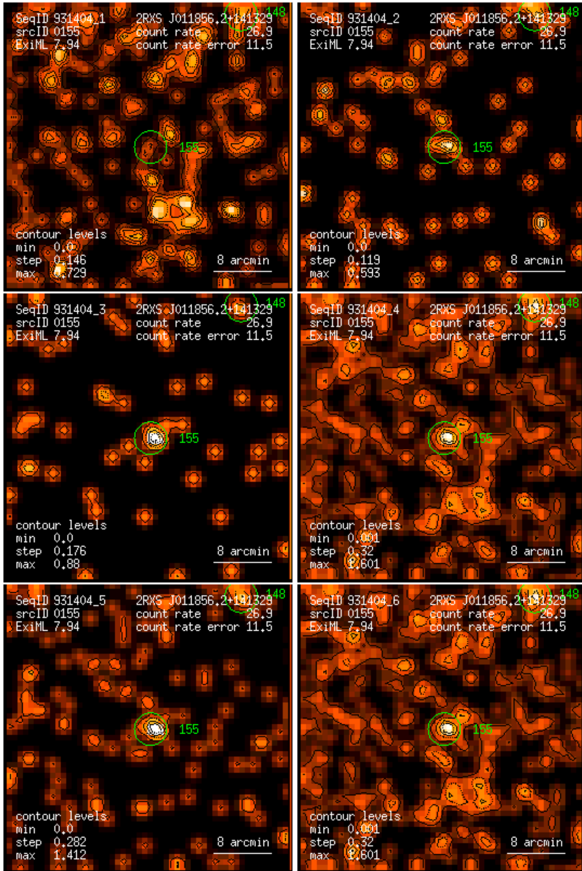
Figure 155: RASS 931404: detection 0155: band rate images, Gaussian filter: (1) PSPC channels 11 – 41, (2) 52 – 90, (3) 91 – 201, (4) 11 – 235, (5) 52 – 201, (6) 11 – 201. Broad band rates in counts/ks. Band rate contour levels in counts/ks/arcmin 2 .
