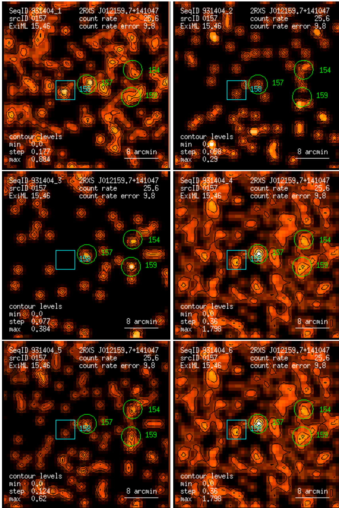
Figure 157: RASS 931404: detection 0157: band rate images, Gaussian filter: (1) PSPC channels 11 – 41, (2) 52 – 90, (3) 91 – 201, (4) 11 – 235, (5) 52 – 201, (6) 11 – 201. Broad band rates in counts/ks. Band rate contour levels in counts/ks/arcmin 2 .
