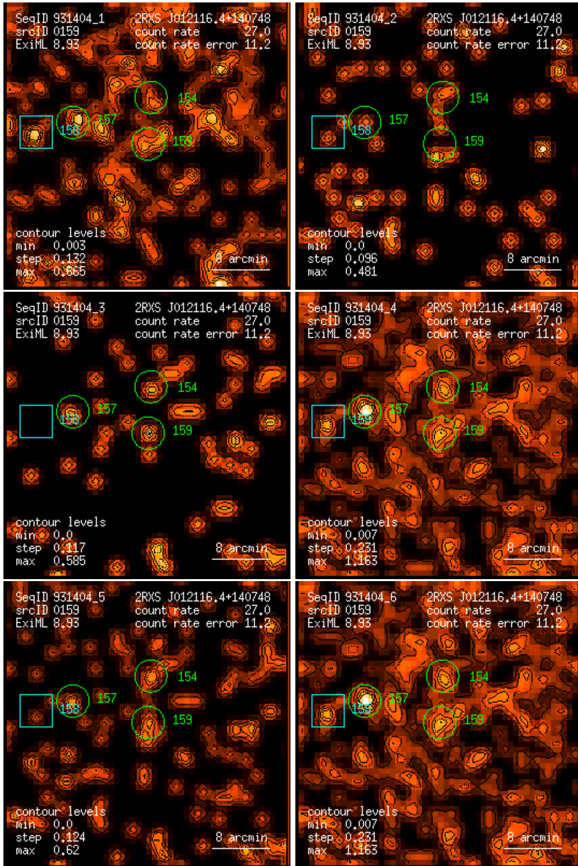
Figure 159: RASS 931404: detection 0159: band rate images, Gaussian filter: (1) PSPC channels 11 – 41, (2) 52 – 90, (3) 91 – 201, (4) 11 – 235, (5) 52 – 201, (6) 11 – 201. Broad band rates in counts/ks. Band rate contour levels in counts/ks/arcmin 2 .
