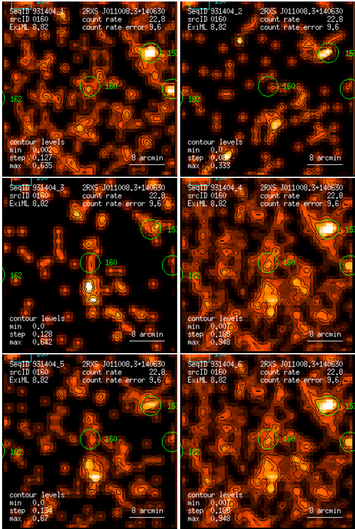
Figure 160: RASS 931404: detection 0160: band rate images, Gaussian filter: (1) PSPC channels 11 – 41, (2) 52 – 90, (3) 91 – 201, (4) 11 – 235, (5) 52 – 201, (6) 11 – 201. Broad band rates in counts/ks. Band rate contour levels in counts/ks/arcmin 2 .
