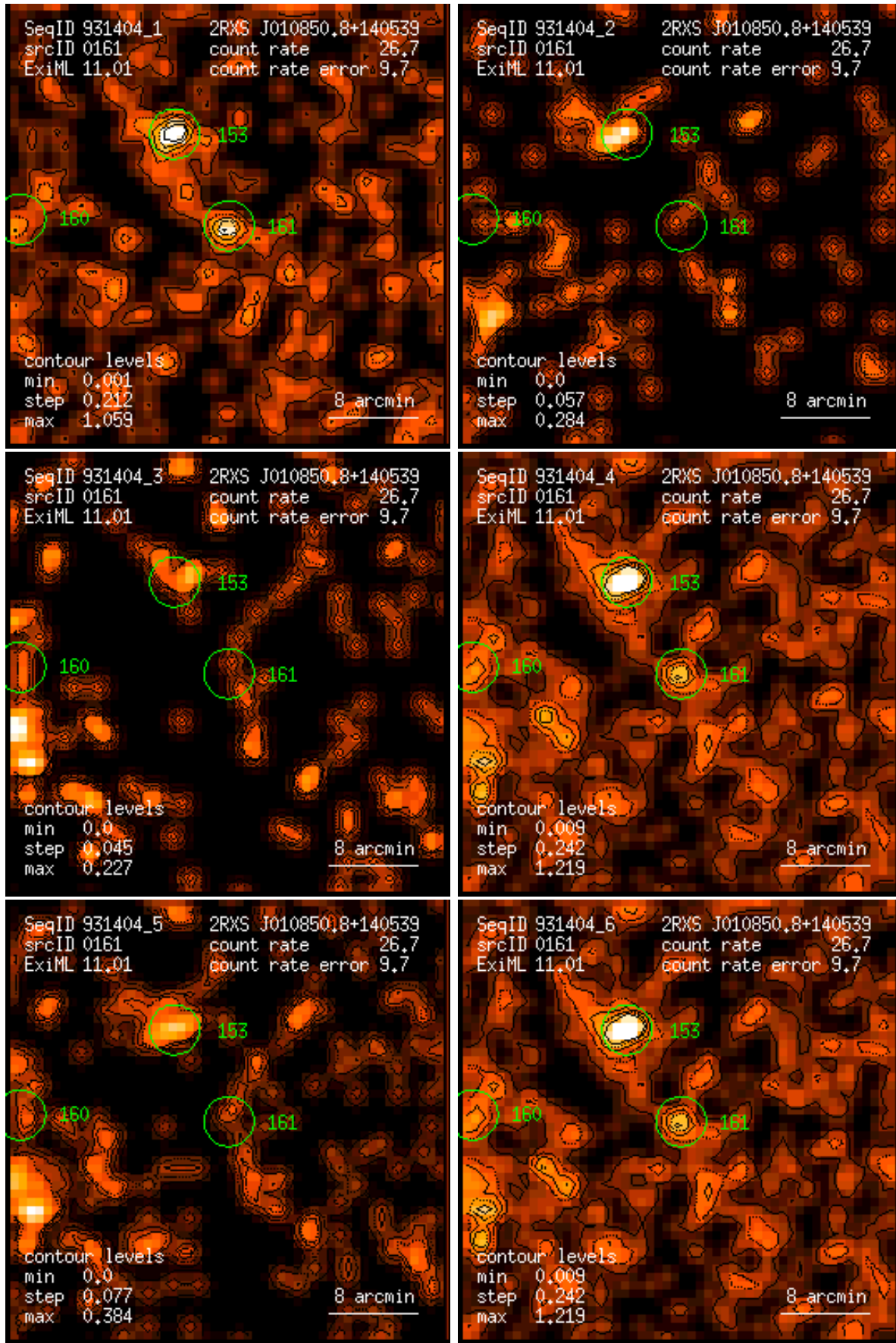
Figure 161: RASS 931404: detection 0161: band rate images, Gaussian filter: (1) PSPC channels 11 – 41, (2) 52 – 90, (3) 91 – 201, (4) 11 – 235, (5) 52 – 201, (6) 11 – 201. Broad band rates in counts/ks. Band rate contour levels in counts/ks/arcmin 2 .
