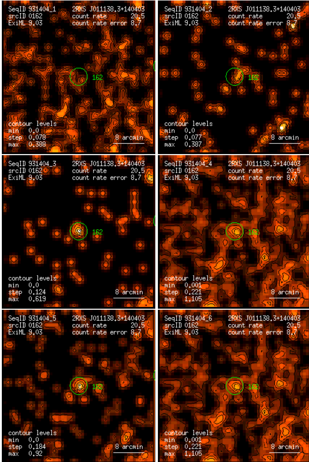
Figure 162: RASS 931404: detection 0162: band rate images, Gaussian filter: (1) PSPC channels 11 – 41, (2) 52 – 90, (3) 91 – 201, (4) 11 – 235, (5) 52 – 201, (6) 11 – 201. Broad band rates in counts/ks. Band rate contour levels in counts/ks/arcmin 2 .
