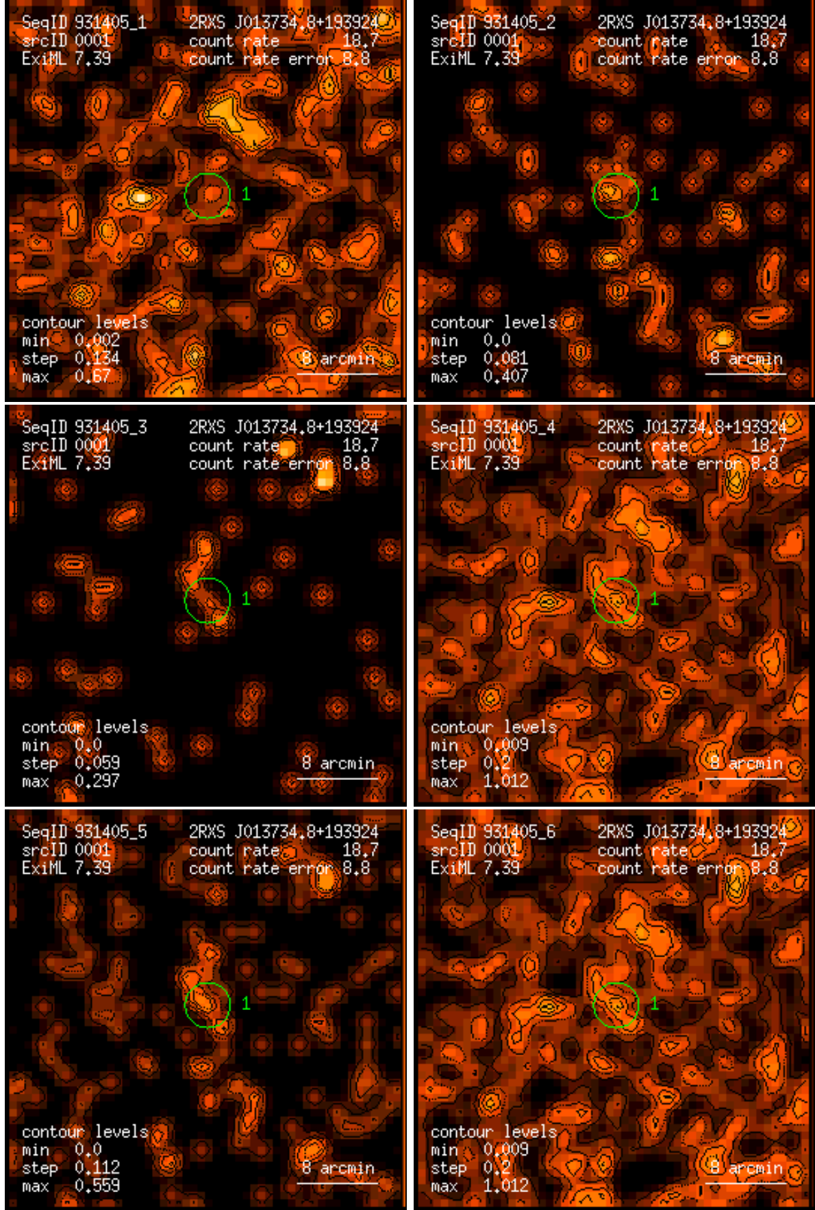
Figure 1: RASS 931405: detection 0001: band rate images, Gaussian filter: (1) PSPC channels 11 – 41, (2) 52 – 90, (3) 91 – 201, (4) 11 – 235, (5) 52 – 201, (6) 11 – 201. Broad band rates in counts/ks. Band rate contour levels in counts/ks/arcmin 2 .
