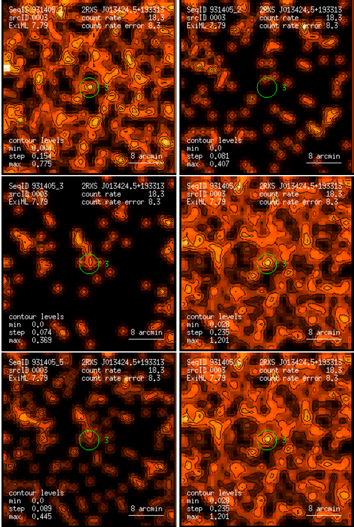
Figure 3: RASS 931405: detection 0003: band rate images, Gaussian filter: (1) PSPC channels 11 – 41, (2) 52 – 90, (3) 91 – 201, (4) 11 – 235, (5) 52 – 201, (6) 11 – 201. Broad band rates in counts/ks. Band rate contour levels in counts/ks/arcmin 2 .
