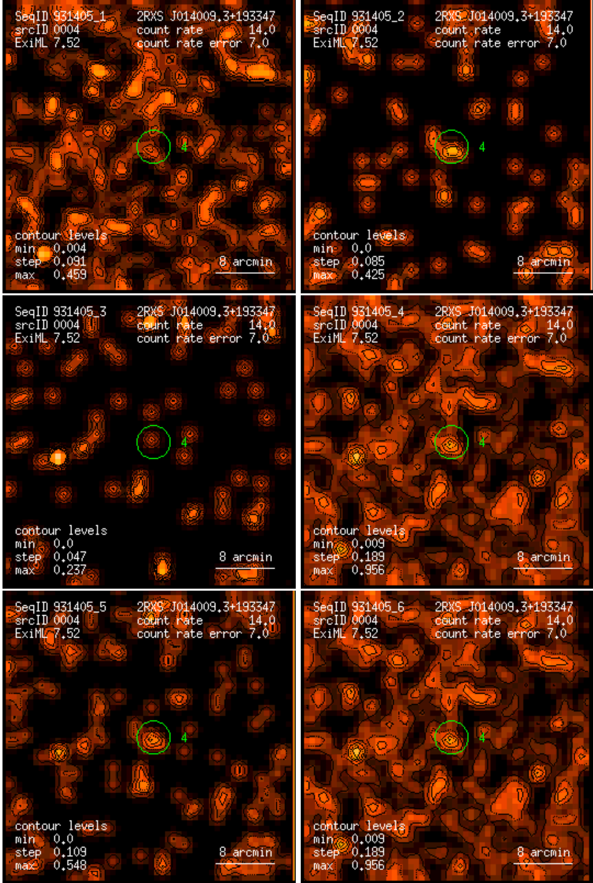
Figure 4: RASS 931405: detection 0004: band rate images, Gaussian filter: (1) PSPC channels 11 – 41, (2) 52 – 90, (3) 91 – 201, (4) 11 – 235, (5) 52 – 201, (6) 11 – 201. Broad band rates in counts/ks. Band rate contour levels in counts/ks/arcmin 2 .
