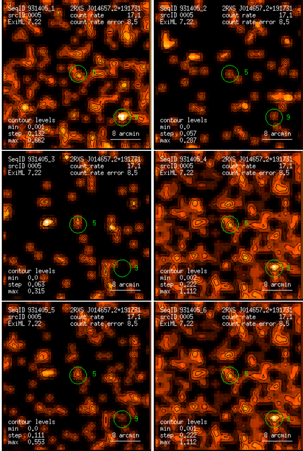
Figure 5: RASS 931405: detection 0005: band rate images, Gaussian filter: (1) PSPC channels 11 – 41, (2) 52 – 90, (3) 91 – 201, (4) 11 – 235, (5) 52 – 201, (6) 11 – 201. Broad band rates in counts/ks. Band rate contour levels in counts/ks/arcmin 2 .
