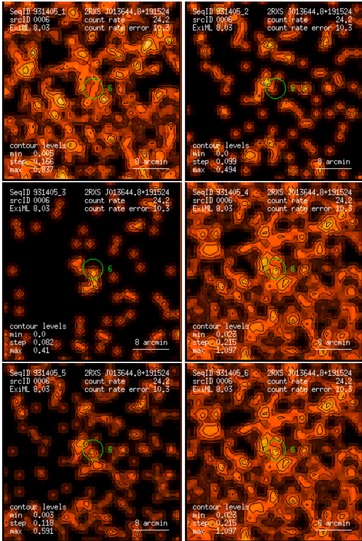
Figure 6: RASS 931405: detection 0006: band rate images, Gaussian filter: (1) PSPC channels 11 – 41, (2) 52 – 90, (3) 91 – 201, (4) 11 – 235, (5) 52 – 201, (6) 11 – 201. Broad band rates in counts/ks. Band rate contour levels in counts/ks/arcmin 2 .
