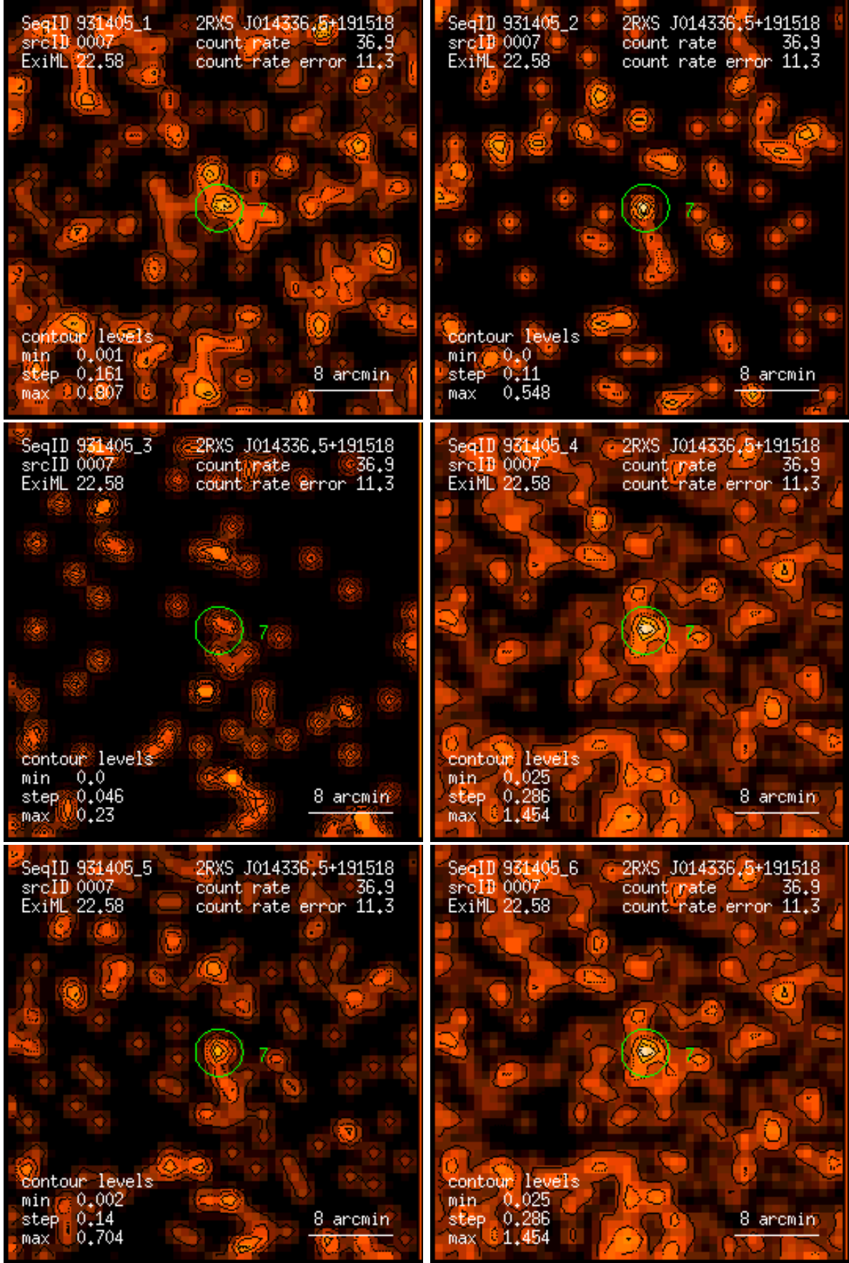
Figure 7: RASS 931405: detection 0007: band rate images, Gaussian filter: (1) PSPC channels 11 – 41, (2) 52 – 90, (3) 91 – 201, (4) 11 – 235, (5) 52 – 201, (6) 11 – 201. Broad band rates in counts/ks. Band rate contour levels in counts/ks/arcmin 2 .
