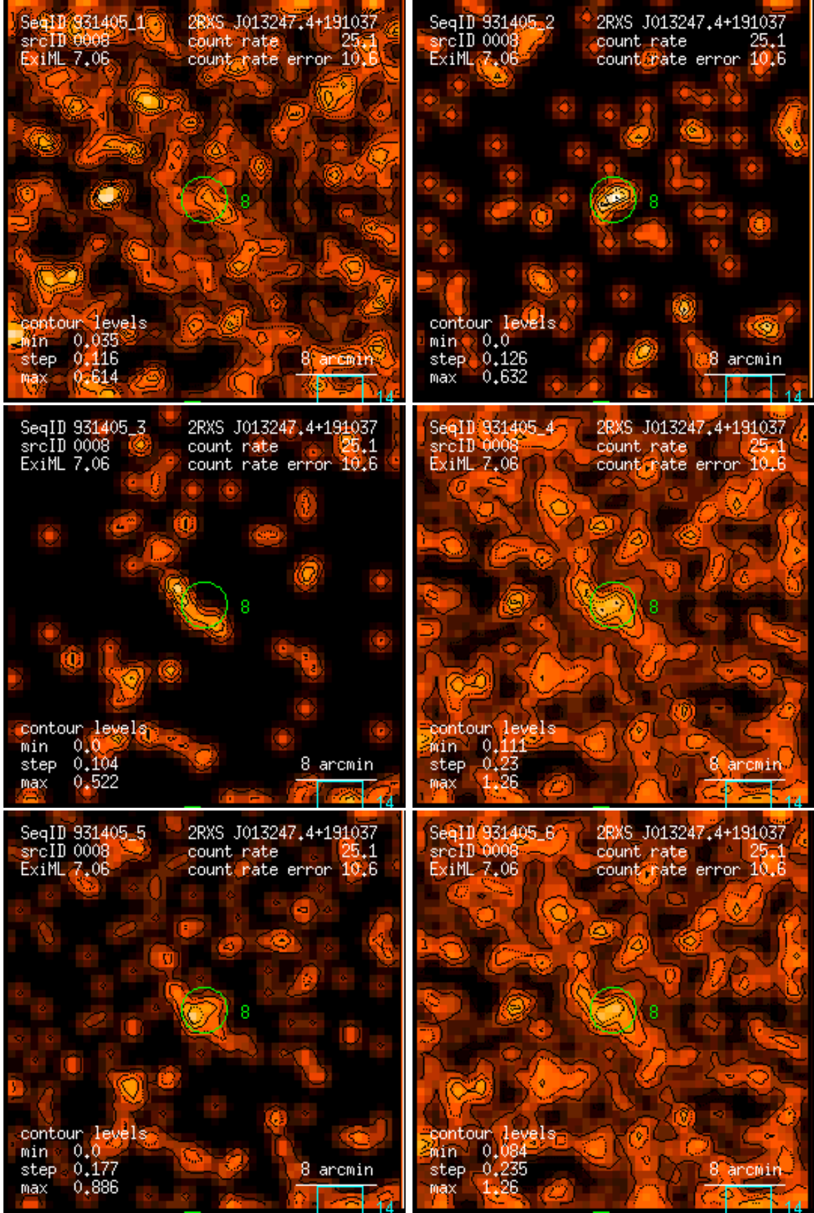
Figure 8: RASS 931405: detection 0008: band rate images, Gaussian filter: (1) PSPC channels 11 – 41, (2) 52 – 90, (3) 91 – 201, (4) 11 – 235, (5) 52 – 201, (6) 11 – 201. Broad band rates in counts/ks. Band rate contour levels in counts/ks/arcmin 2 .
