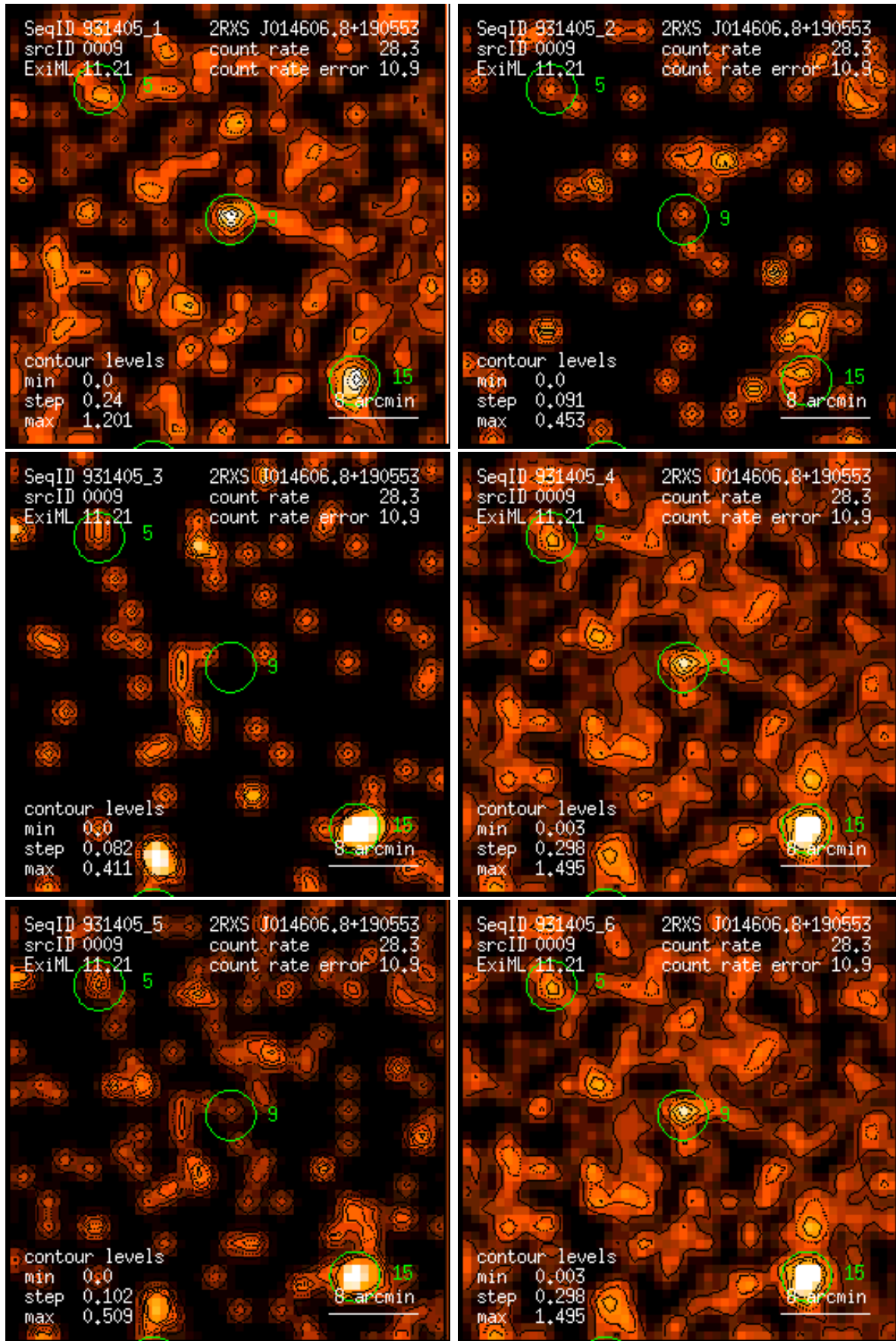
Figure 9: RASS 931405: detection 0009: band rate images, Gaussian filter: (1) PSPC channels 11 – 41, (2) 52 – 90, (3) 91 – 201, (4) 11 – 235, (5) 52 – 201, (6) 11 – 201. Broad band rates in counts/ks. Band rate contour levels in counts/ks/arcmin 2 .
