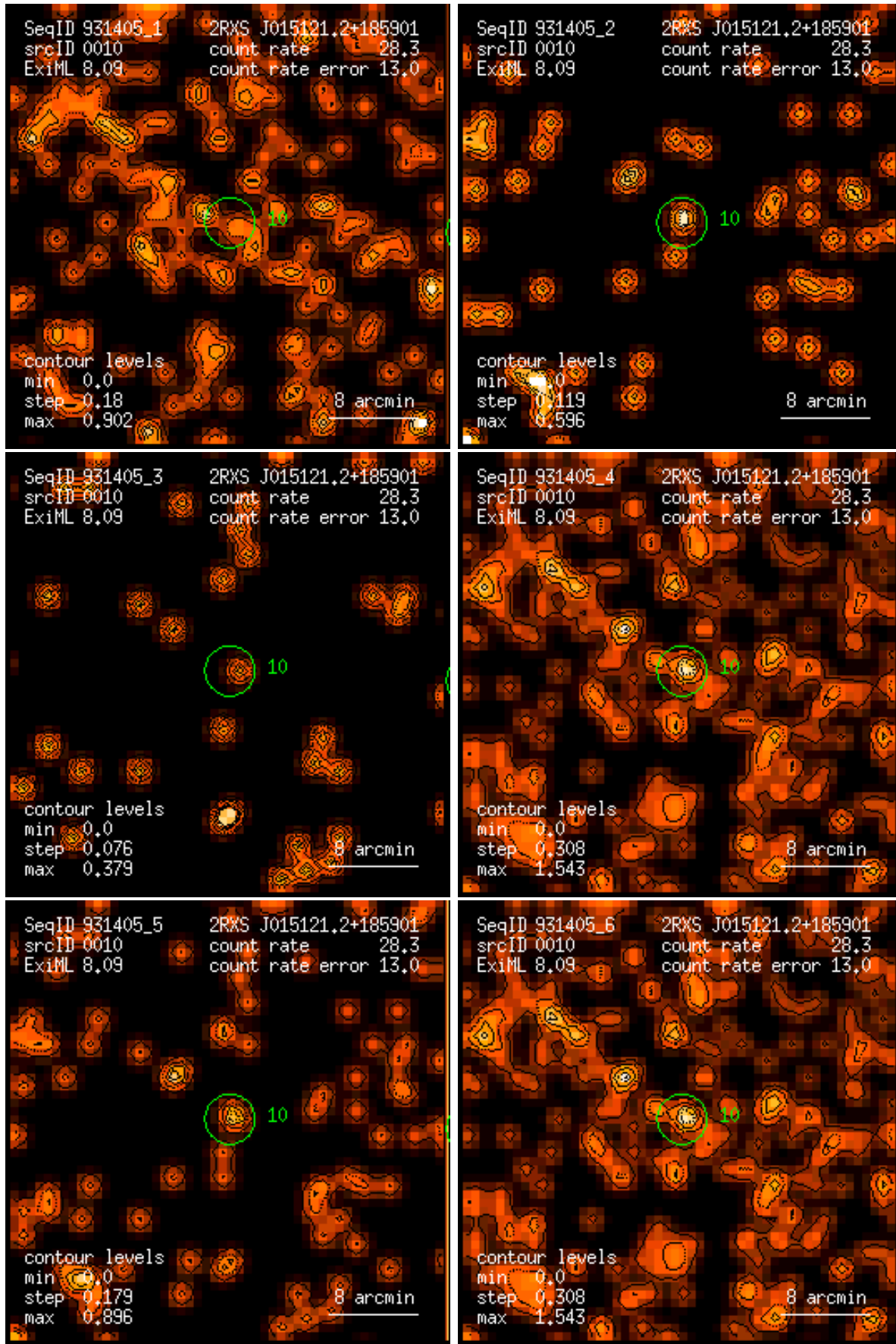
Figure 10: RASS 931405: detection 0010: band rate images, Gaussian filter: (1) PSPC channels 11 – 41, (2) 52 – 90, (3) 91 – 201, (4) 11 – 235, (5) 52 – 201, (6) 11 – 201. Broad band rates in counts/ks. Band rate contour levels in counts/ks/arcmin 2 .
