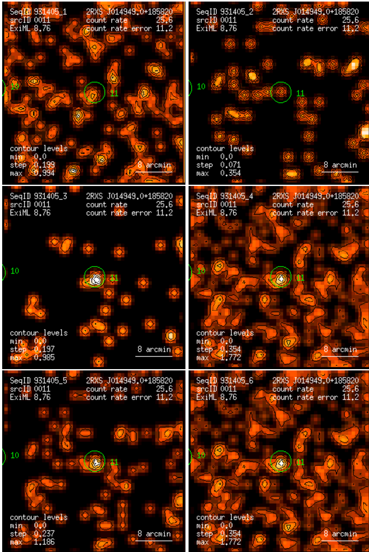
Figure 11: RASS 931405: detection 0011: band rate images, Gaussian filter: (1) PSPC channels 11 – 41, (2) 52 – 90, (3) 91 – 201, (4) 11 – 235, (5) 52 – 201, (6) 11 – 201. Broad band rates in counts/ks. Band rate contour levels in counts/ks/arcmin 2 .
