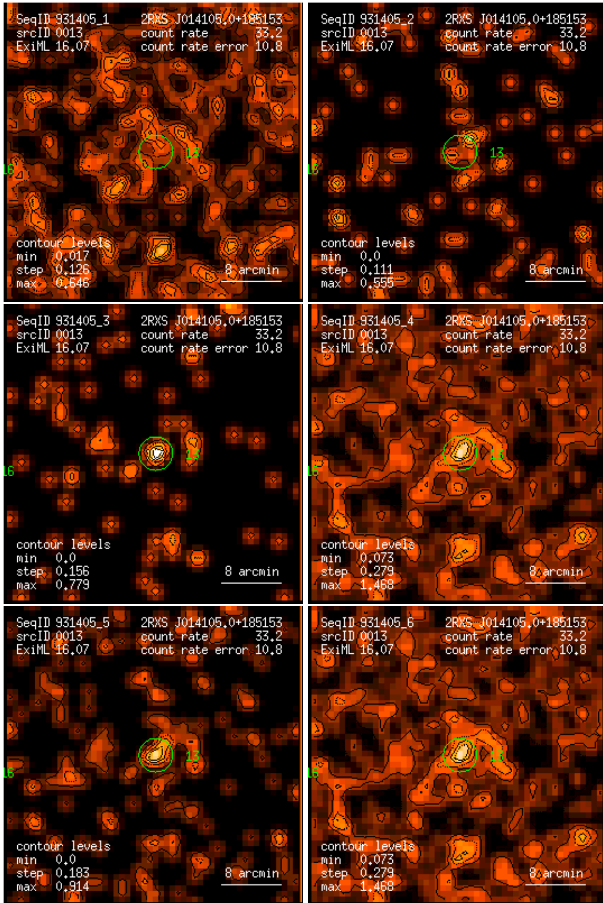
Figure 13: RASS 931405: detection 0013: band rate images, Gaussian filter: (1) PSPC channels 11 – 41, (2) 52 – 90, (3) 91 – 201, (4) 11 – 235, (5) 52 – 201, (6) 11 – 201. Broad band rates in counts/ks. Band rate contour levels in counts/ks/arcmin 2 .
