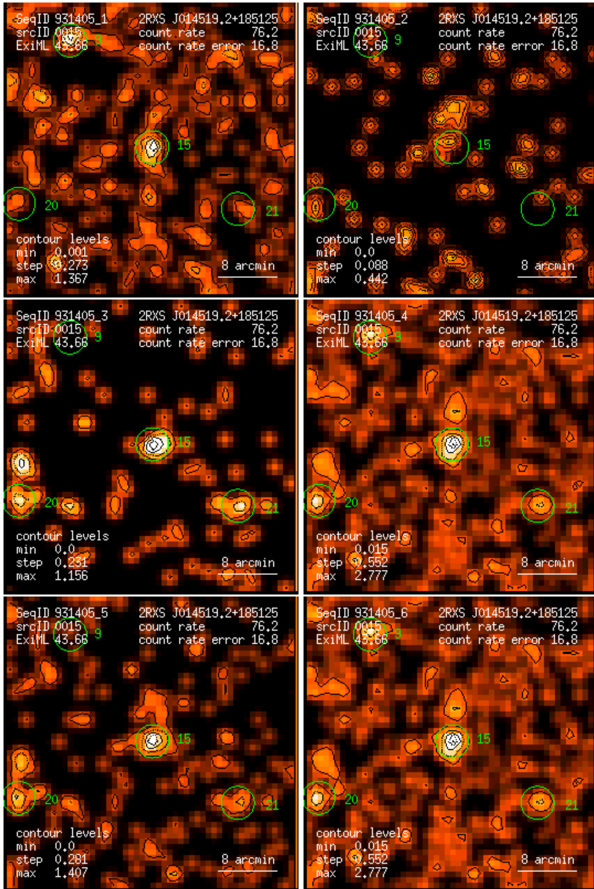
Figure 15: RASS 931405: detection 0015: band rate images, Gaussian filter: (1) PSPC channels 11 – 41, (2) 52 – 90, (3) 91 – 201, (4) 11 – 235, (5) 52 – 201, (6) 11 – 201. Broad band rates in counts/ks. Band rate contour levels in counts/ks/arcmin 2 .
