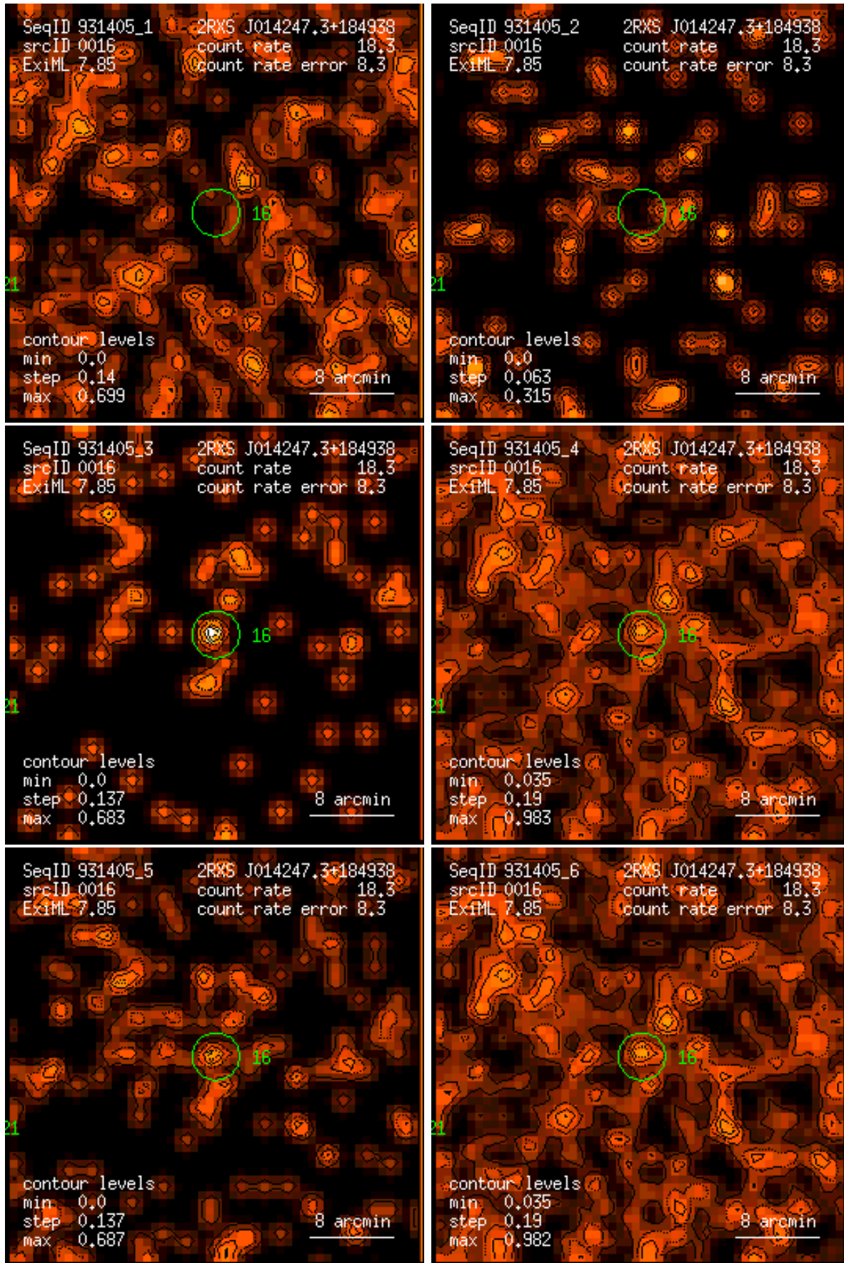
Figure 16: RASS 931405: detection 0016: band rate images, Gaussian filter: (1) PSPC channels 11 – 41, (2) 52 – 90, (3) 91 – 201, (4) 11 – 235, (5) 52 – 201, (6) 11 – 201. Broad band rates in counts/ks. Band rate contour levels in counts/ks/arcmin 2 .
