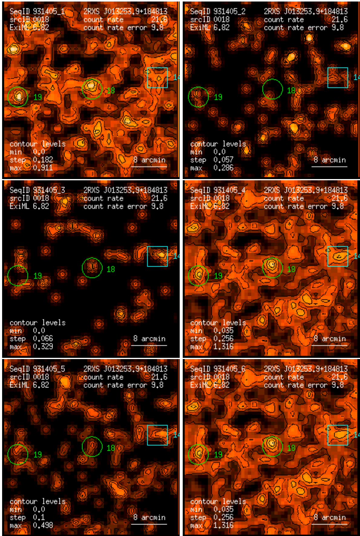
Figure 18: RASS 931405: detection 0018: band rate images, Gaussian filter: (1) PSPC channels 11 – 41, (2) 52 – 90, (3) 91 – 201, (4) 11 – 235, (5) 52 – 201, (6) 11 – 201. Broad band rates in counts/ks. Band rate contour levels in counts/ks/arcmin 2 .
