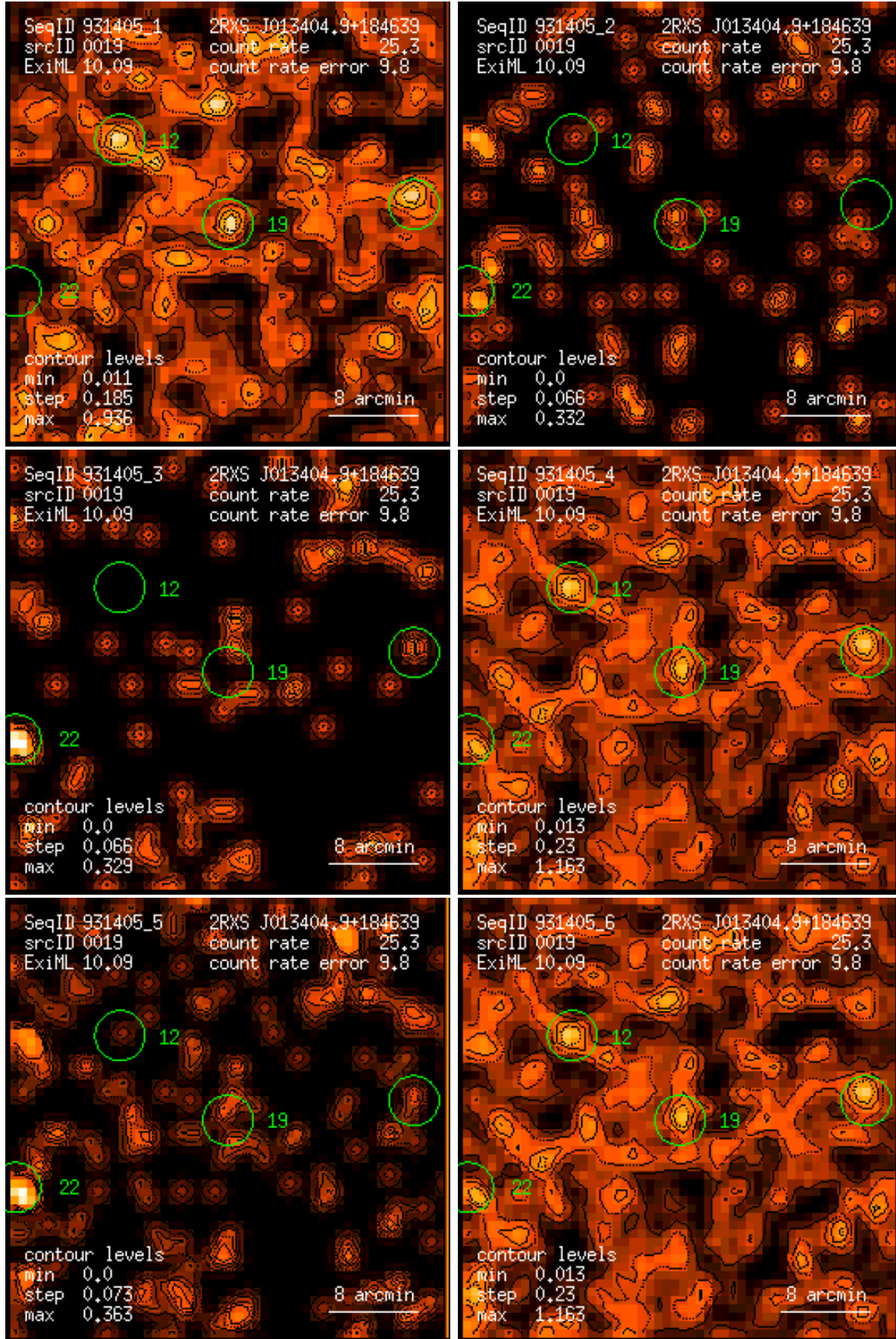
Figure 19: RASS 931405: detection 0019: band rate images, Gaussian filter: (1) PSPC channels 11 – 41, (2) 52 – 90, (3) 91 – 201, (4) 11 – 235, (5) 52 – 201, (6) 11 – 201. Broad band rates in counts/ks. Band rate contour levels in counts/ks/arcmin 2 .
