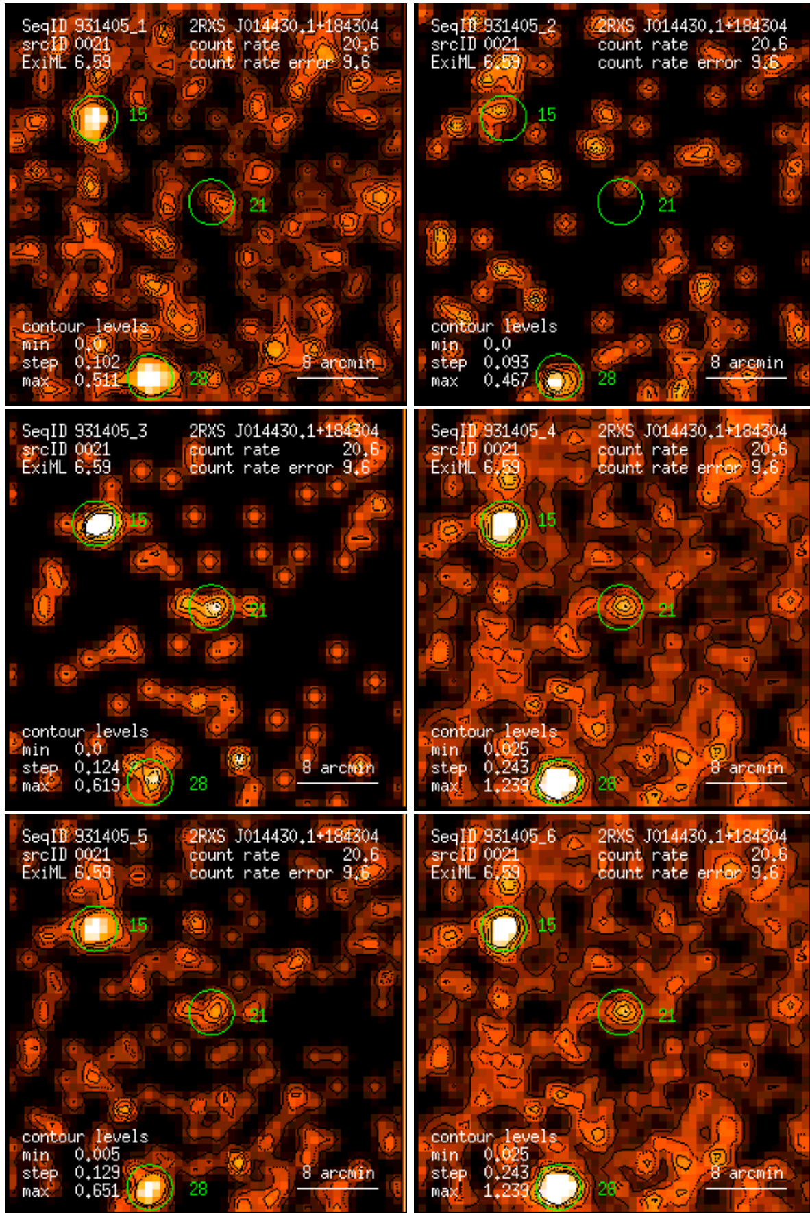
Figure 21: RASS 931405: detection 0021: band rate images, Gaussian filter: (1) PSPC channels 11 – 41, (2) 52 – 90, (3) 91 – 201, (4) 11 – 235, (5) 52 – 201, (6) 11 – 201. Broad band rates in counts/ks. Band rate contour levels in counts/ks/arcmin 2 .
