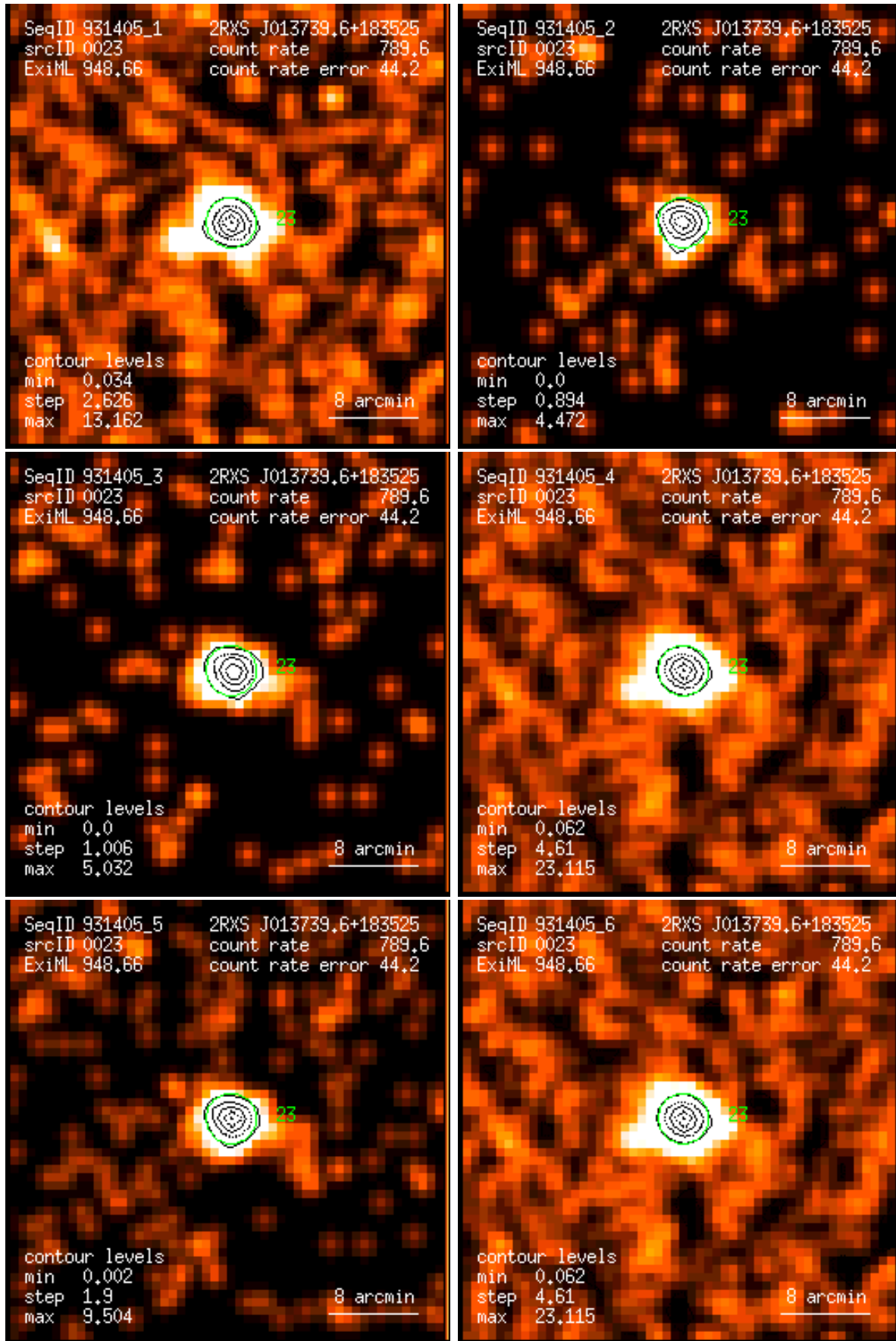
Figure 23: RASS 931405: detection 0023: band rate images, Gaussian filter: (1) PSPC channels 11 – 41, (2) 52 – 90, (3) 91 – 201, (4) 11 – 235, (5) 52 – 201, (6) 11 – 201. Broad band rates in counts/ks. Band rate contour levels in counts/ks/arcmin 2 .
