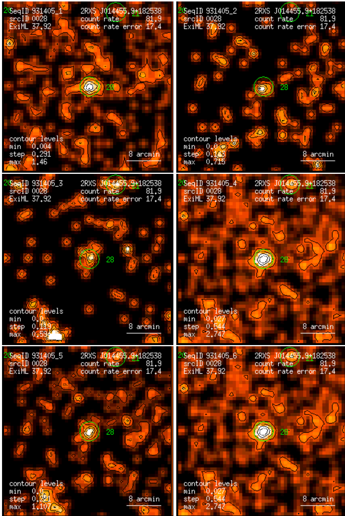
Figure 28: RASS 931405: detection 0028: band rate images, Gaussian filter: (1) PSPC channels 11 – 41, (2) 52 – 90, (3) 91 – 201, (4) 11 – 235, (5) 52 – 201, (6) 11 – 201. Broad band rates in counts/ks. Band rate contour levels in counts/ks/arcmin 2 .
