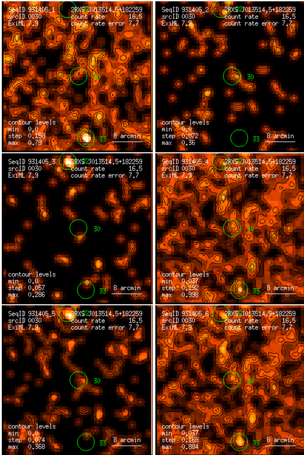
Figure 30: RASS 931405: detection 0030: band rate images, Gaussian filter: (1) PSPC channels 11 – 41, (2) 52 – 90, (3) 91 – 201, (4) 11 – 235, (5) 52 – 201, (6) 11 – 201. Broad band rates in counts/ks. Band rate contour levels in counts/ks/arcmin 2 .
