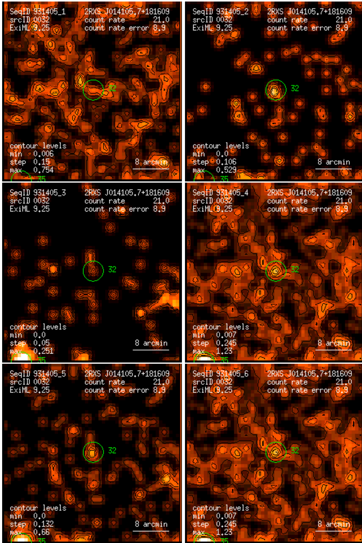
Figure 32: RASS 931405: detection 0032: band rate images, Gaussian filter: (1) PSPC channels 11 – 41, (2) 52 – 90, (3) 91 – 201, (4) 11 – 235, (5) 52 – 201, (6) 11 – 201. Broad band rates in counts/ks. Band rate contour levels in counts/ks/arcmin 2 .
