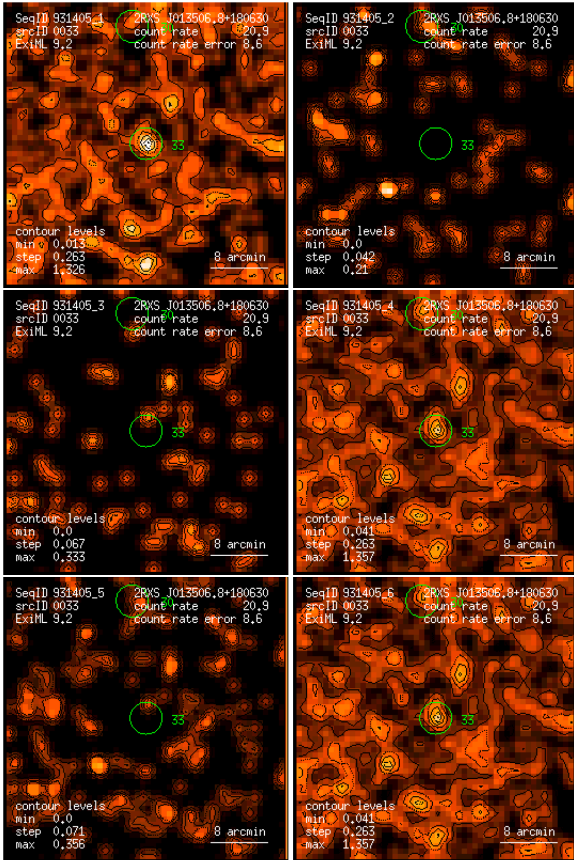
Figure 33: RASS 931405: detection 0033: band rate images, Gaussian filter: (1) PSPC channels 11 – 41, (2) 52 – 90, (3) 91 – 201, (4) 11 – 235, (5) 52 – 201, (6) 11 – 201. Broad band rates in counts/ks. Band rate contour levels in counts/ks/arcmin 2 .
