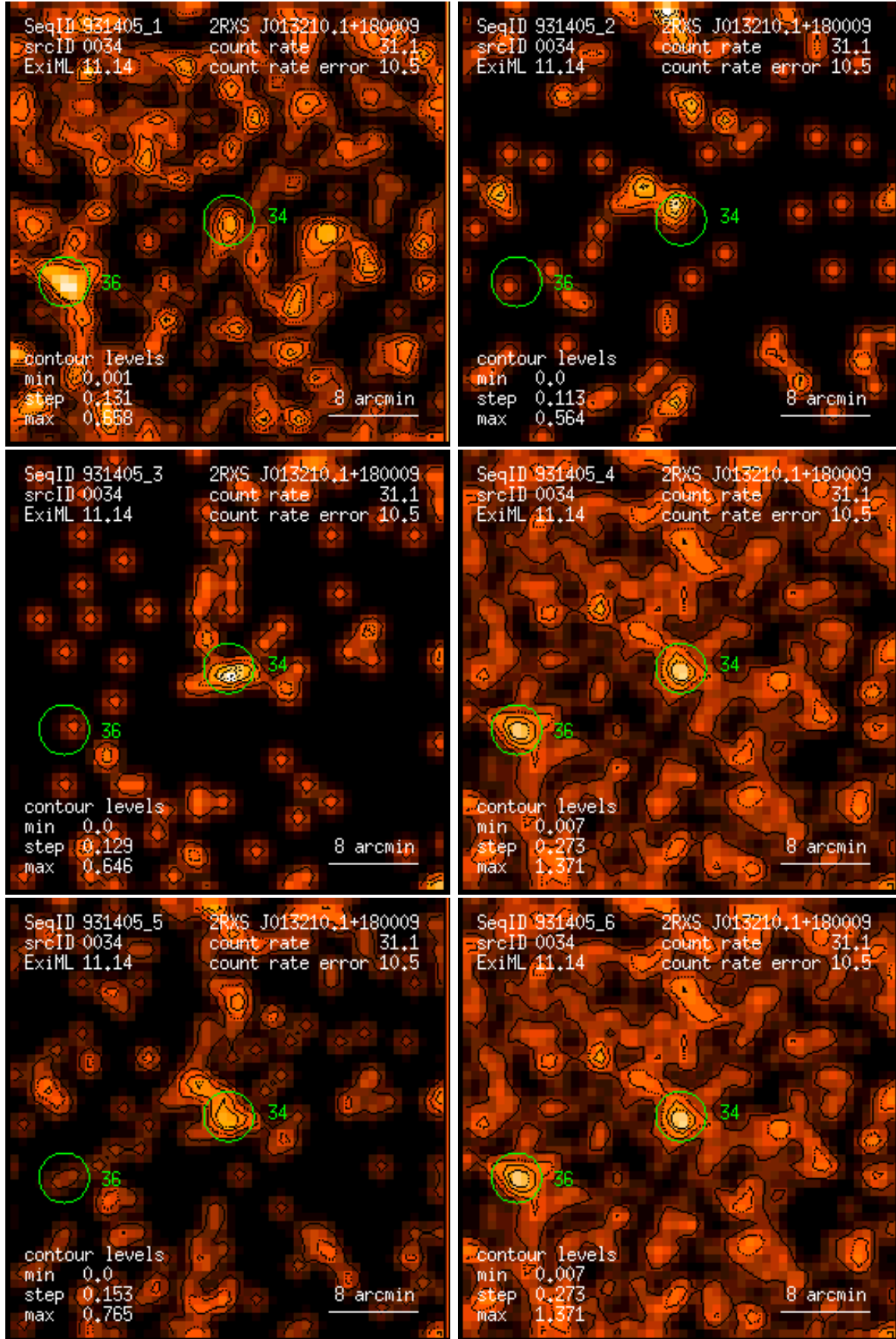
Figure 34: RASS 931405: detection 0034: band rate images, Gaussian filter: (1) PSPC channels 11 – 41, (2) 52 – 90, (3) 91 – 201, (4) 11 – 235, (5) 52 – 201, (6) 11 – 201. Broad band rates in counts/ks. Band rate contour levels in counts/ks/arcmin 2 .
