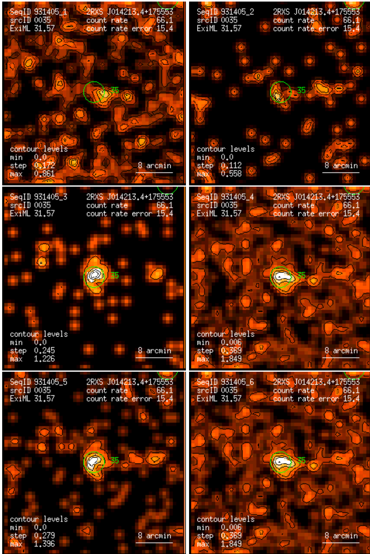
Figure 35: RASS 931405: detection 0035: band rate images, Gaussian filter: (1) PSPC channels 11 – 41, (2) 52 – 90, (3) 91 – 201, (4) 11 – 235, (5) 52 – 201, (6) 11 – 201. Broad band rates in counts/ks. Band rate contour levels in counts/ks/arcmin 2 .
